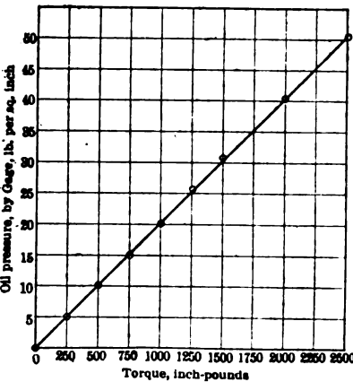
Fig. 4—Calibration curve for transmission dynamometer.
